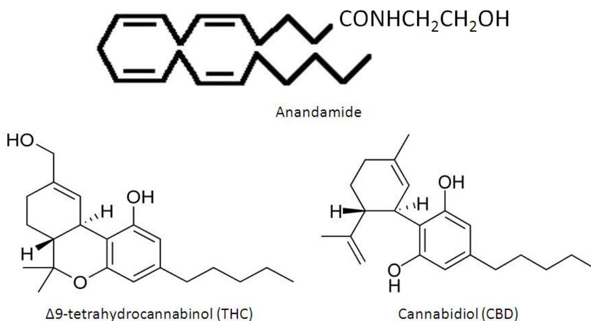
Figure 3. Chemical Structures of Anandamide, \Delta^9 -Tetrahydrocannabinol, and Cannabidiol.
